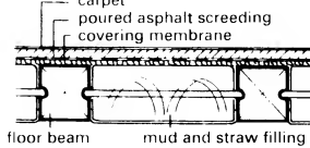
(impact sound insulating floor construction with poured asphalt screeding)
